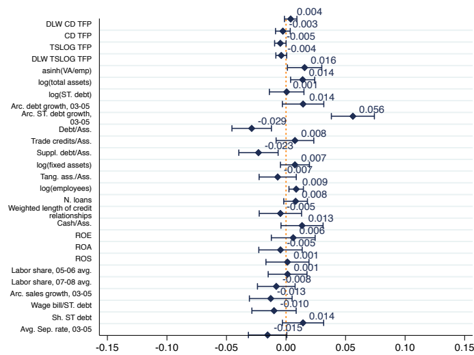
Figure 2: Balance checks
